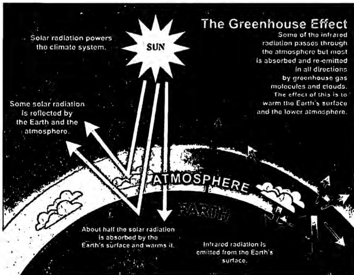
Figure 2-1: The Greenhouse Effect
