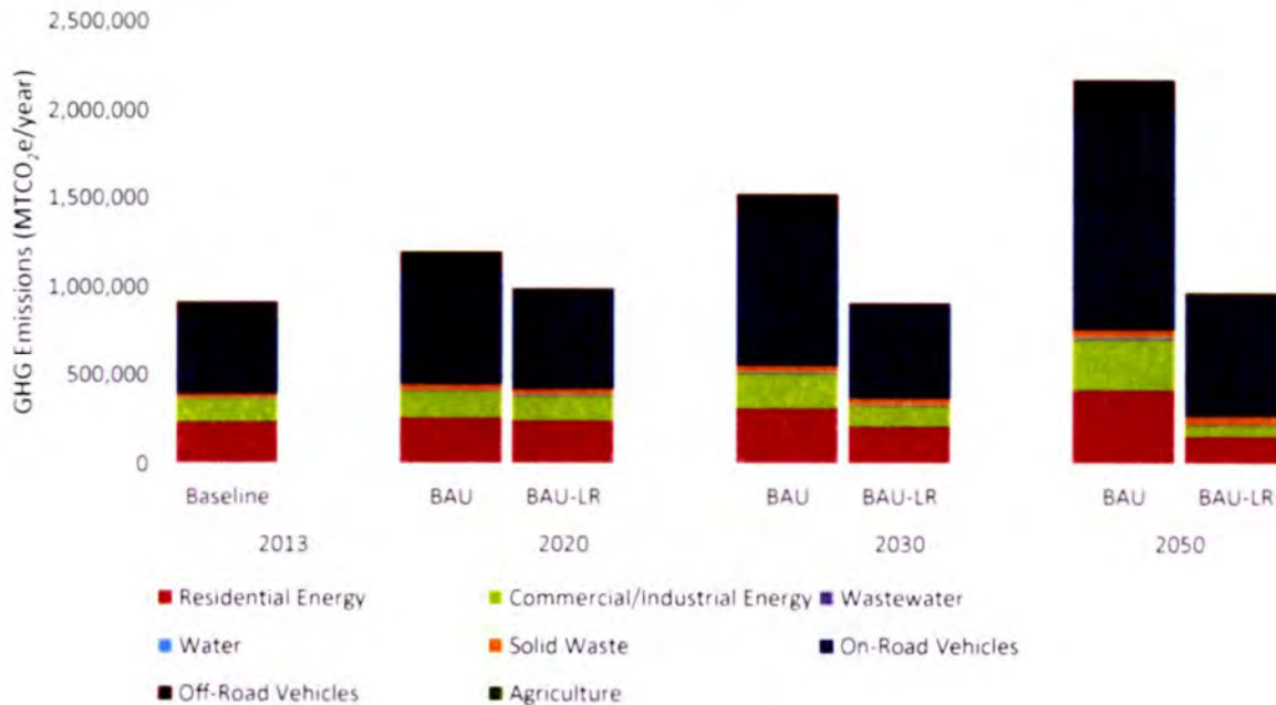
Figure 3-2: Business-as-Usual Emission Forecast by Sector – 2020, 2030 and 2050
