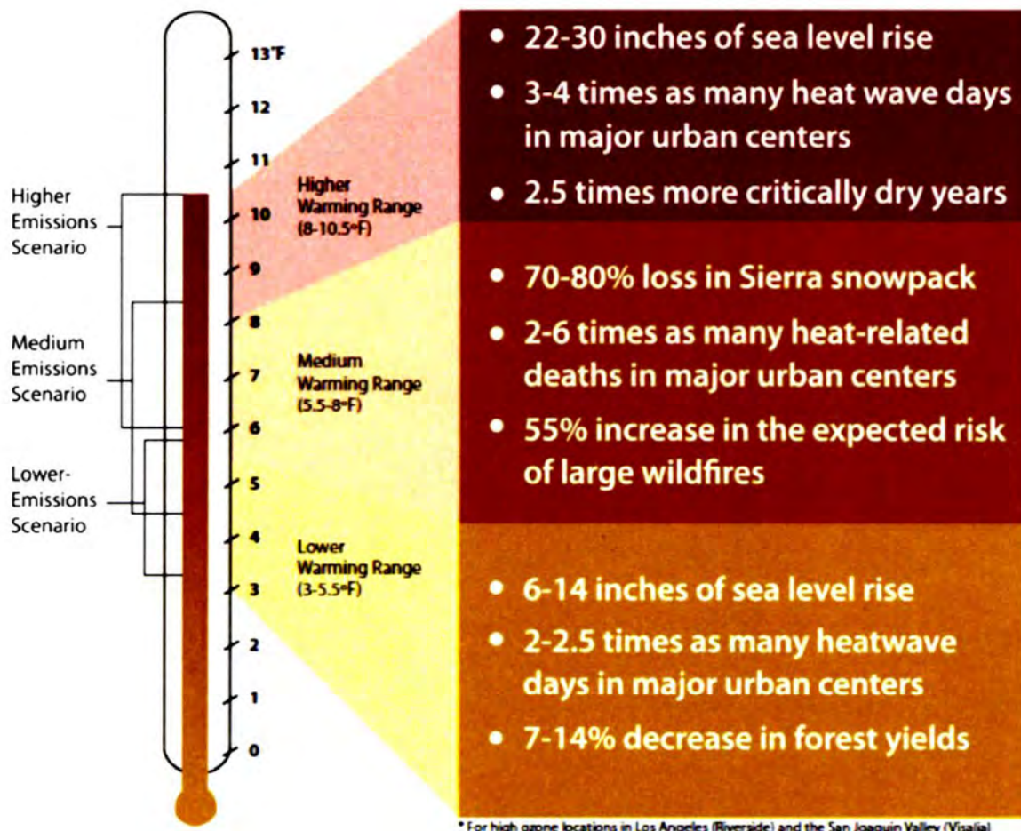
Figure 2-2: California Climate Change Impacts 9
